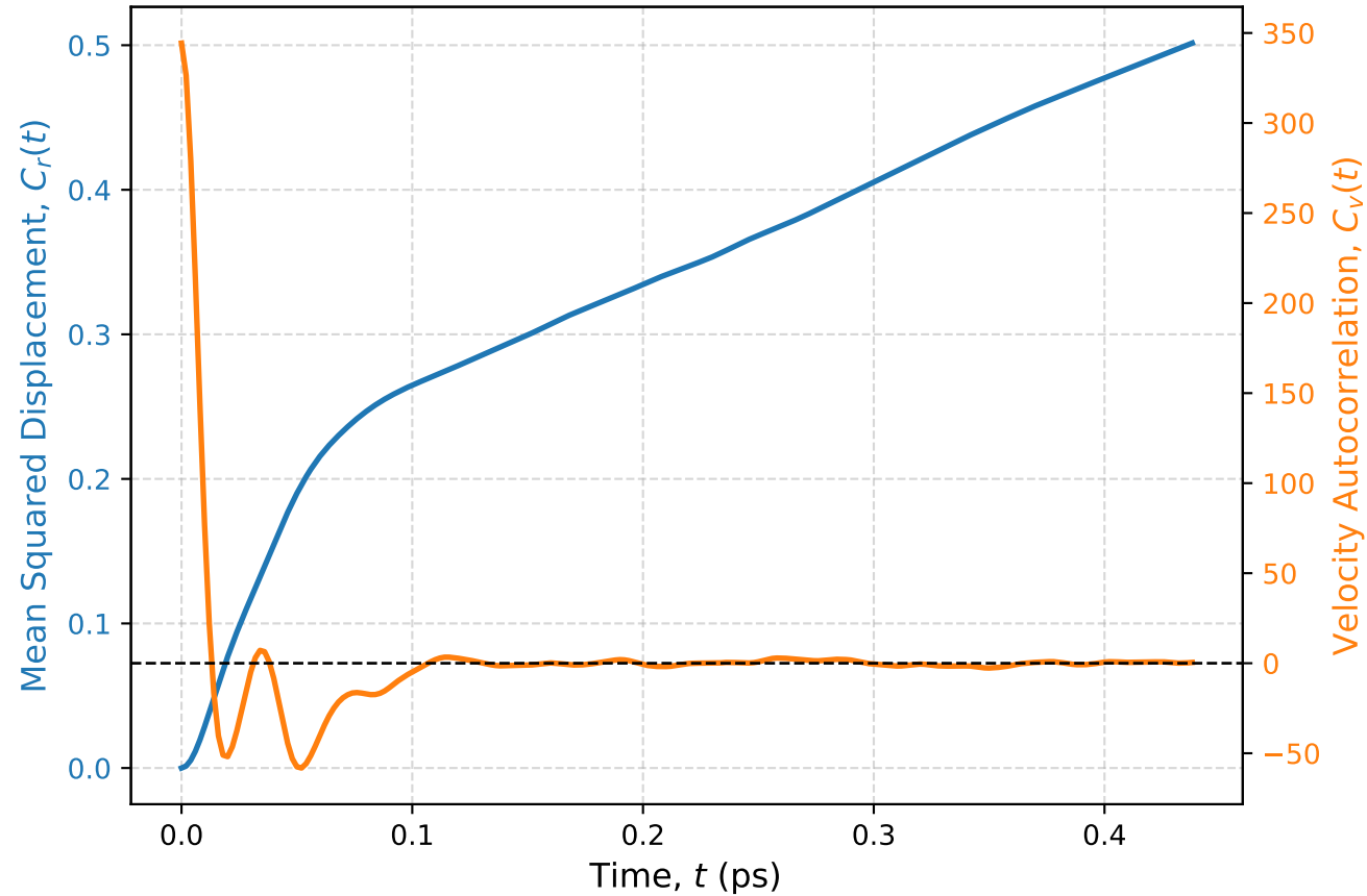
Single-Particle Dynamics (SiC MEAM)
