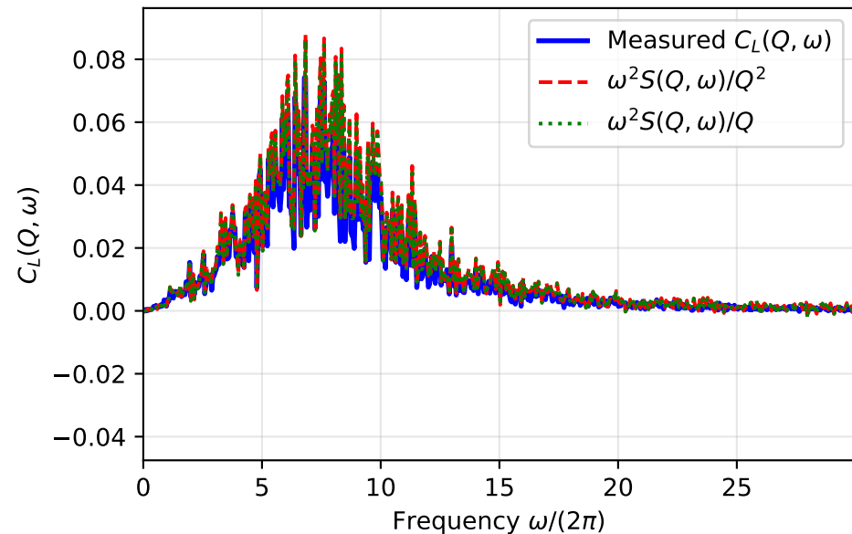
Collective Longitudinal C_L(Q, \omega) ( Q = 0.977 )
