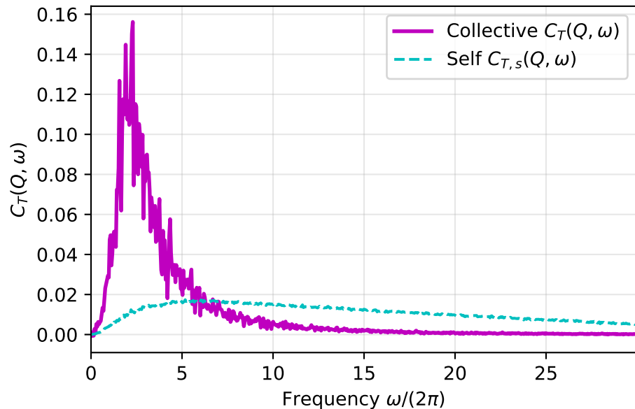
Transverse Current C_T(Q, \omega) ( Q = 0.977 )
