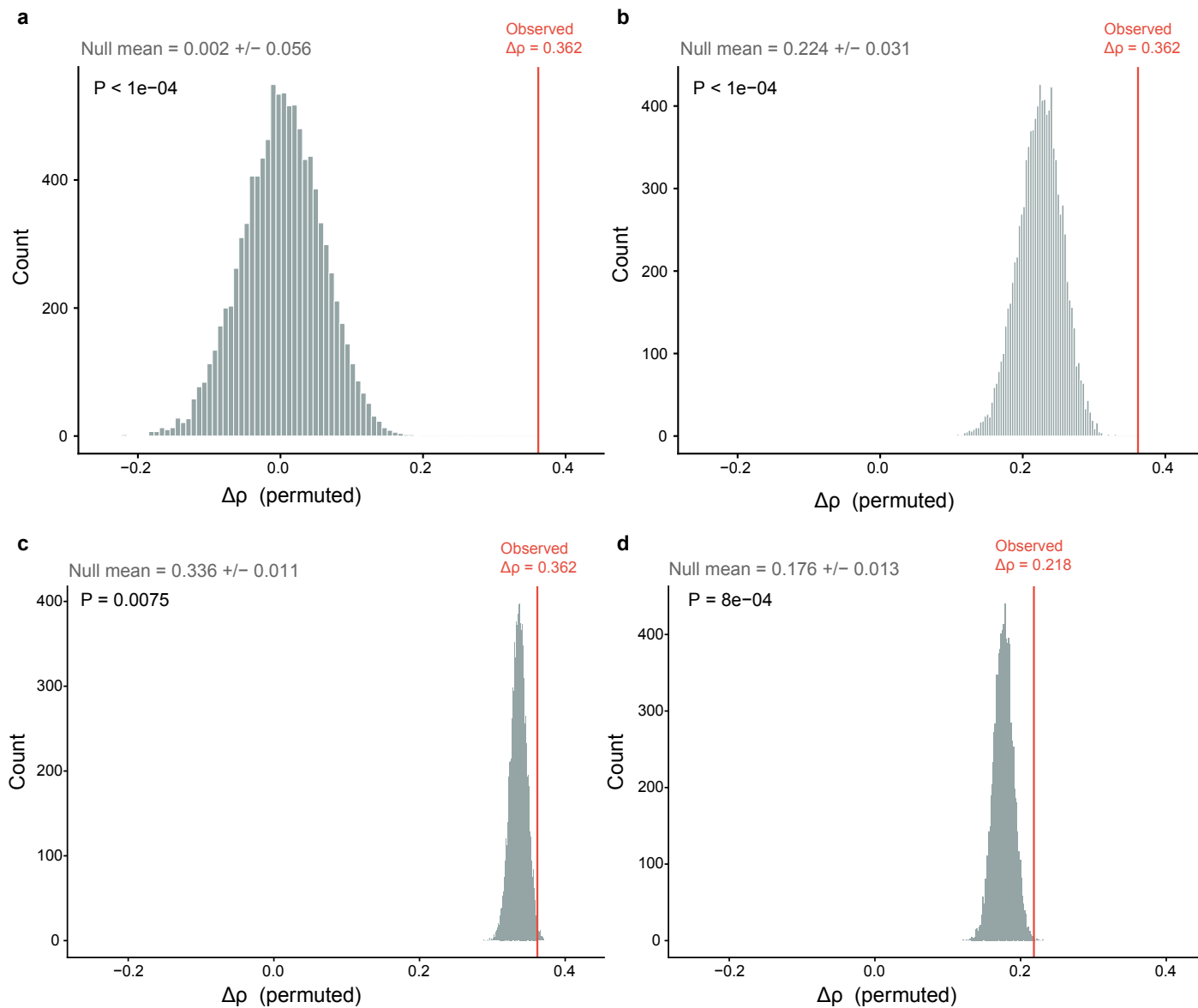
Fig. S5. Permutation and permutation controls for the cross-species fold-change correlation contrast. The observed \Delta\rho (median Spearman \rho of shared DAPs minus background) is shown as a red line in each panel. (a) Naive permutation: shared/background labels shuffled randomly (10,000 replicates). (b) Magnitude-matched permutation: labels shuffled within |\log_2\text{FC}| bins. (c) Brownian-motion (BM) permutation against all background (n = 1,557): for each orthogroup independently, fold-change values were reassigned across species using rank-matched BM simulation along the species phylogeny (10,000 replicates). (d) BM permutation against magnitude-matched single-species DAPs (n = 155; |\log_2\text{FC}| \geq 0.53 ). The observed \Delta\rho in panel (d) is 0.218 because the comparison group is magnitude-matched single-species DAPs rather than all background.
