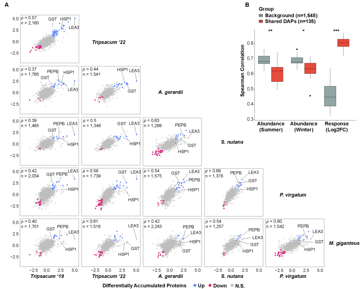
Figure 2. Conservation of seasonal protein accumulation across independently cold-adapted PACMAD grasses. (A) Pairwise comparisons of \log_2 fold-change ( \log_2FC winter/summer) in differentially accumulated orthogroups across species. Scatterplots display the correlation of orthogroup-level \log_2FC values between species, with shared DAPs elevated in winter shown in blue, reduced in red, and non-significant proteins in gray. Each panel represents a comparison between two species, with the number of shared orthogroups ( n ) and Spearman's correlation coefficient ( \rho ) displayed. (B) Pairwise Spearman correlations for orthogroups quantified in at least four of five species, comparing shared DAPs (red; differentially abundant in \geq 2 species) versus background orthogroups (gray; differentially abundant in \leq 1 species). Correlations are shown for summer abundance, winter abundance, and seasonal response magnitude ( \log_2FC winter/summer). Wilcoxon rank-sum test: * P < 0.05 , ** P < 0.01 , *** P < 0.001 .
