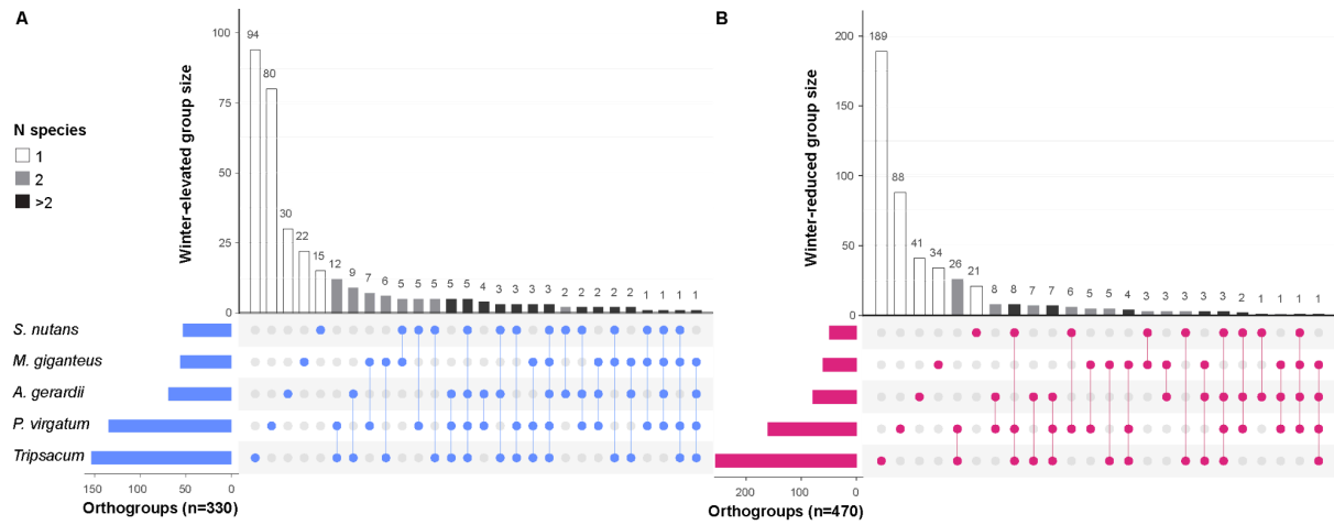
Supplemental Figure S3. Orthogroup sharing of significantly DAPs among five PACMAD grass species. (A) Winter-elevated. (B) Winter-reduced. Set sizes (horizontal bars) indicate the total number of differentially abundant orthogroups identified per species. Intersection sizes (vertical bars) represent orthogroups unique to individual species or shared among multiple species. Bar shading indicates the number of species sharing each orthogroup: unique to one species (white), shared between two species (gray), or shared among more than two species (black). Dots below the plot illustrate species-specific orthogroup intersections.
