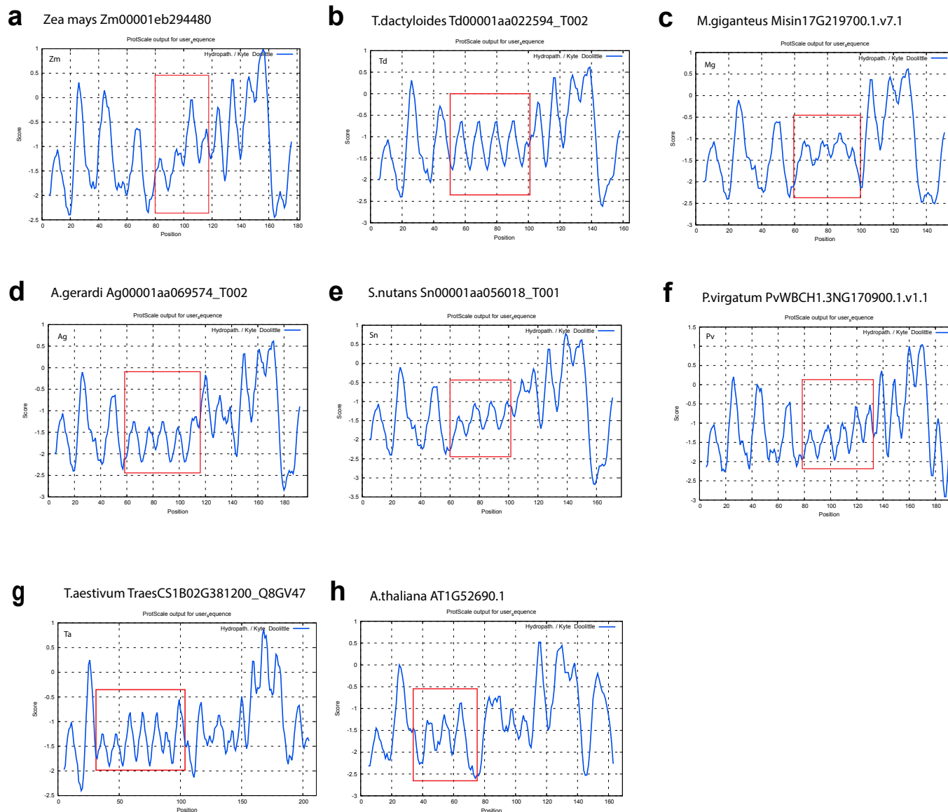
Fig. S9. Hydropathy profiles of LEA3 orthologs. (a) Zea mays , (b) Tripsacum dactyloides , (c) Miscanthus \times giganteus , (d) Andropogon gerardi , (e) Sorghastrum nutans , (f) Panicum virgatum , (g) Triticum aestivum , and (h) Arabidopsis thaliana . Kyte-Doolittle plots were generated using ProtScale (ExPASy) with a window size of 11 amino acids. The x-axis indicates amino acid position, and the y-axis represents hydropathy score. Red boxes indicate the tandem 11-mer repeat region for each species.
