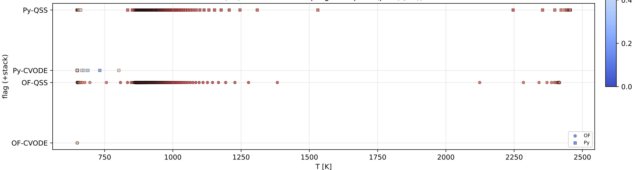
(c) Ignition delay
