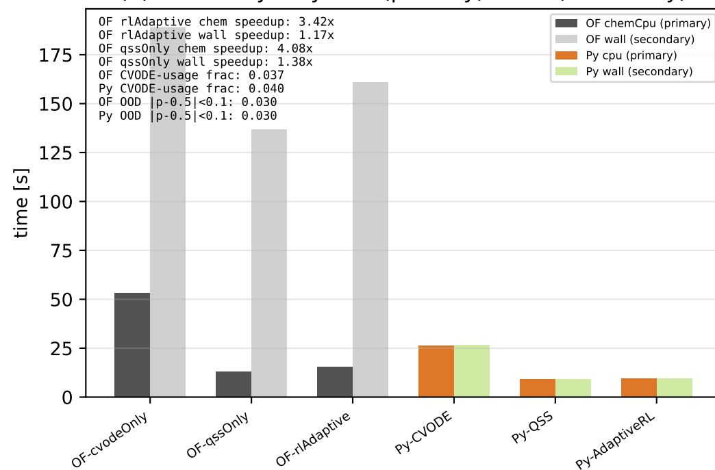
(d) Chemistry-only CPU (primary) / wall (secondary)
