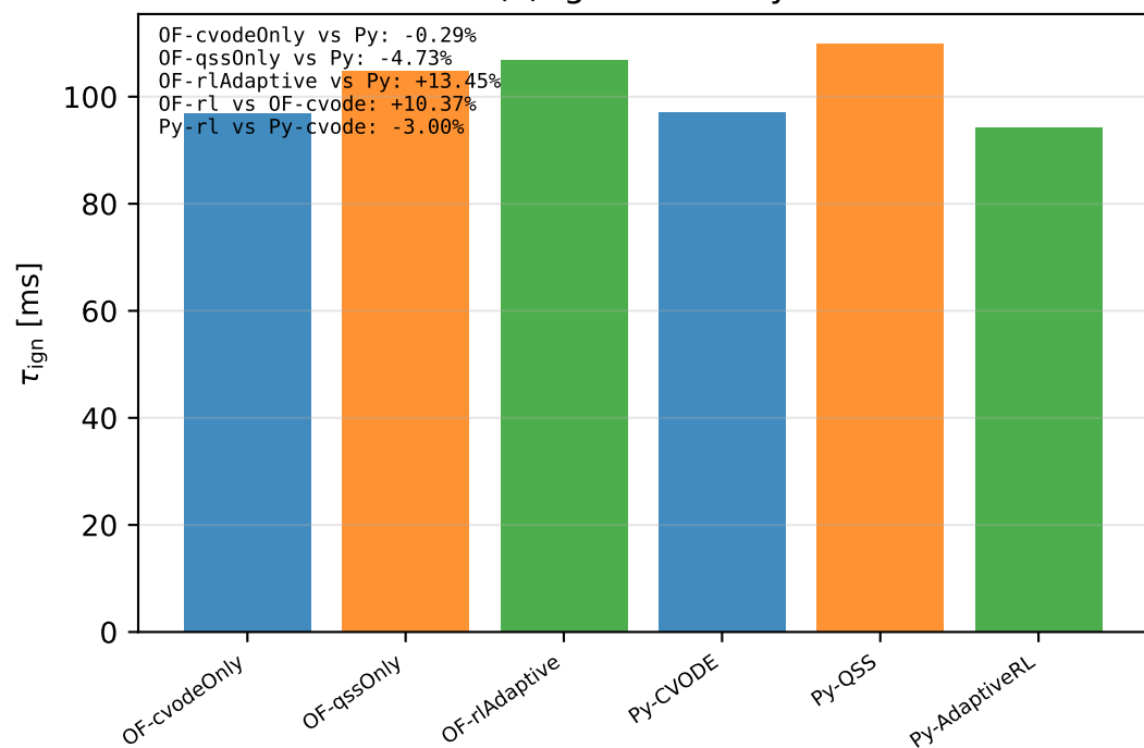
(c) Ignition delay
