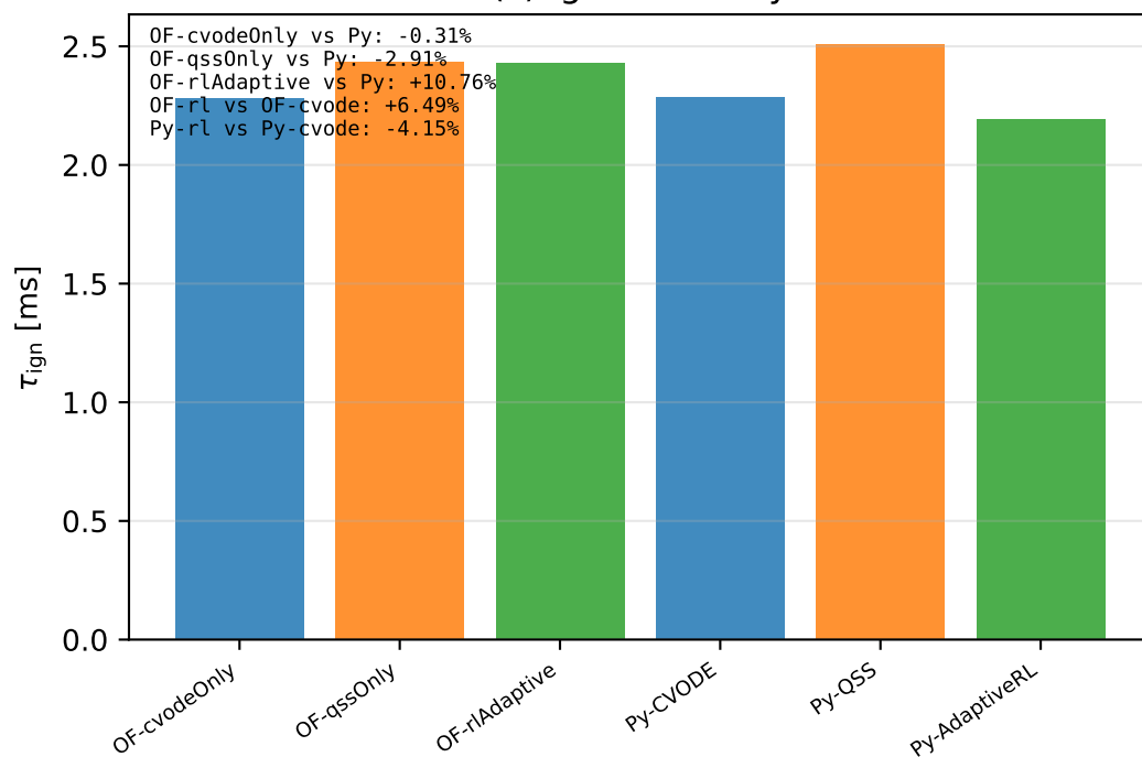
(c) Ignition delay
