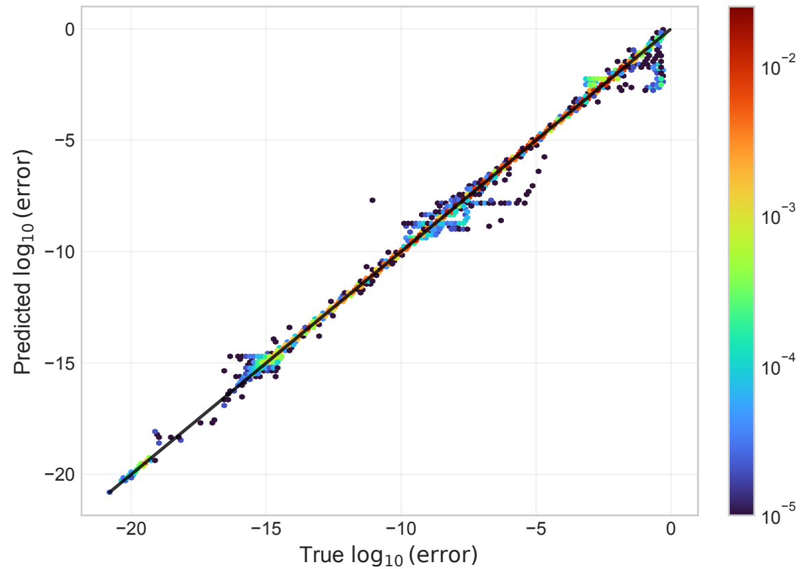
Integrator error ( R^2=1.00 )
