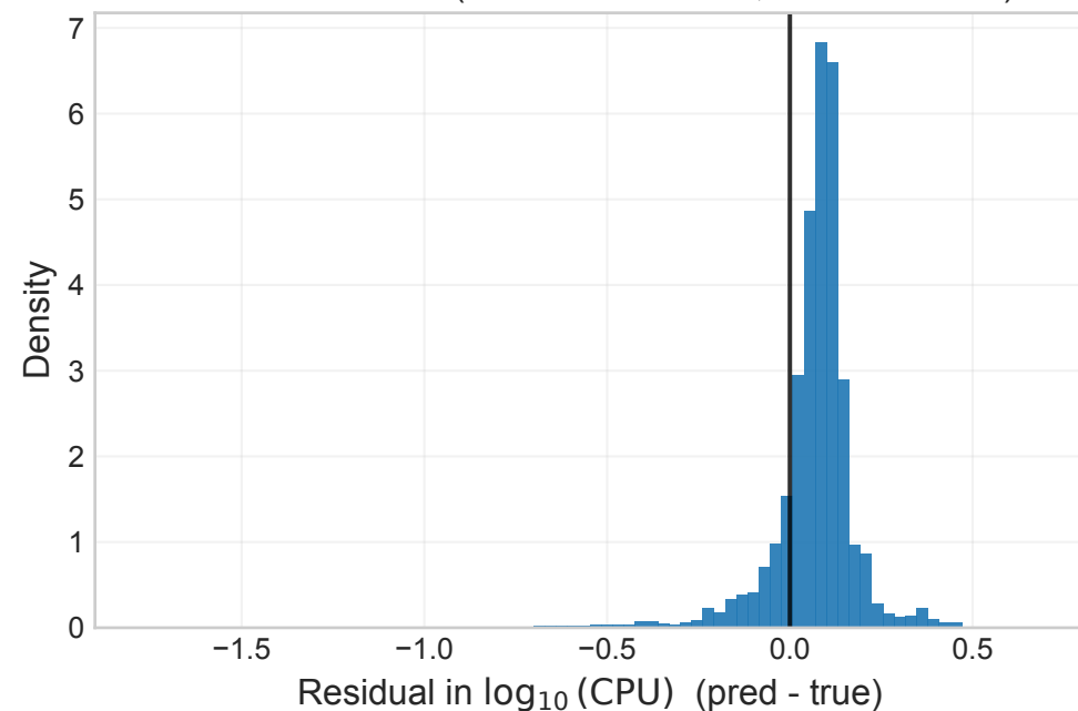
QSS residuals (mean= +1.049\text{e-}01 , std= 2.122\text{e-}01 )
