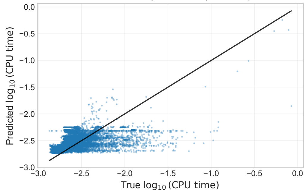
QSS CPU: pred vs true ( R^2=0.040 )
