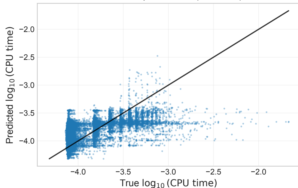
QSS CPU: pred vs true ( R^2=0.040 )
