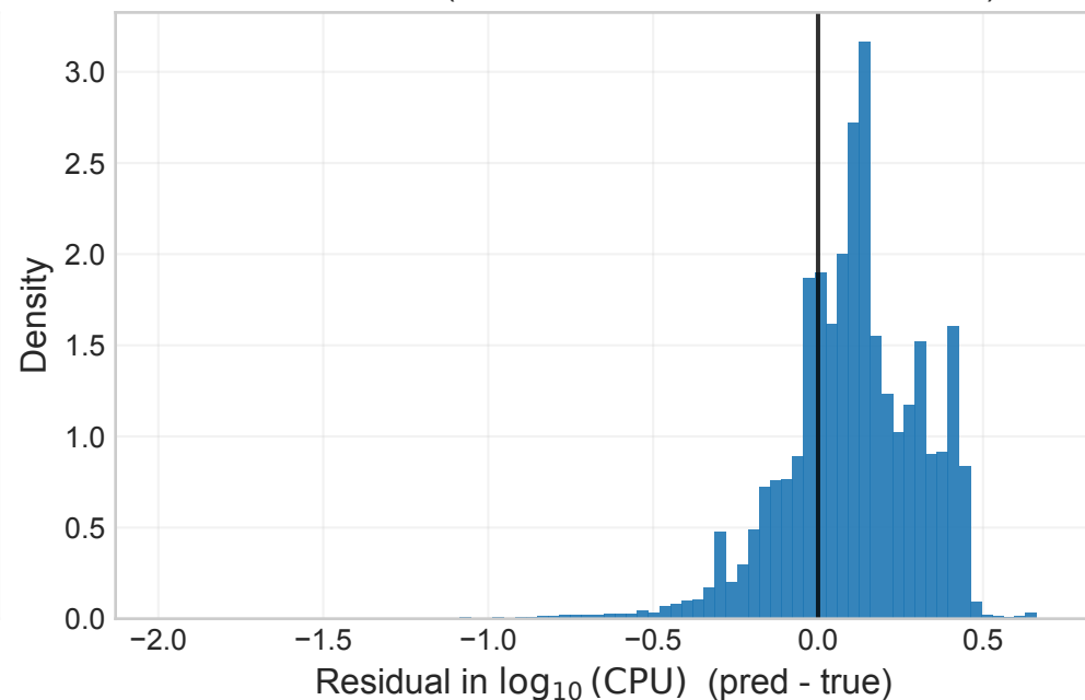
QSS residuals (mean= +1.049\text{e-}01 , std= 2.122\text{e-}01 )
