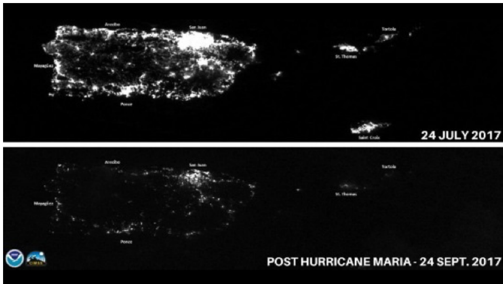
Figure 1: Suomi satellite images of Puerto Rico on 24 July 2017 and 24 September 2017. Image credit: NOAA National Environmental Satellite, Data, and Information Service (NESDIS).
