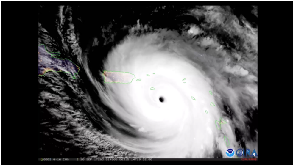
Figure 3: NOAA GOES-16 satellite image of the eye of Hurricane María over Puerto Rico, 20 September 2017.
