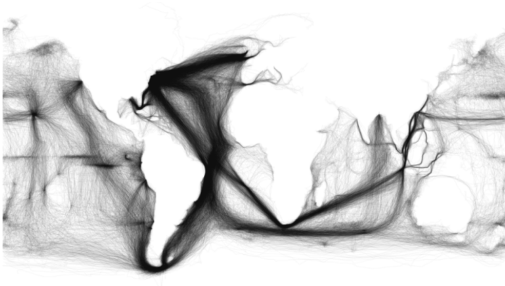
Figure 2: All voyages from the ICOADS US Maury collection. Ships tracks in black, plotted on a white background, show the outlines of the continents and the predominant tracks on the trade winds. Created by Ben Schmidt, 2012.
