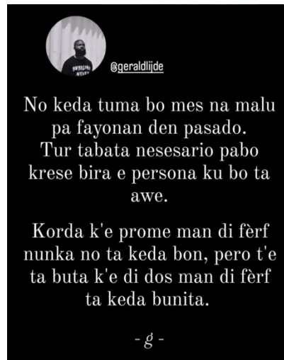
Figure 3: image4.png
