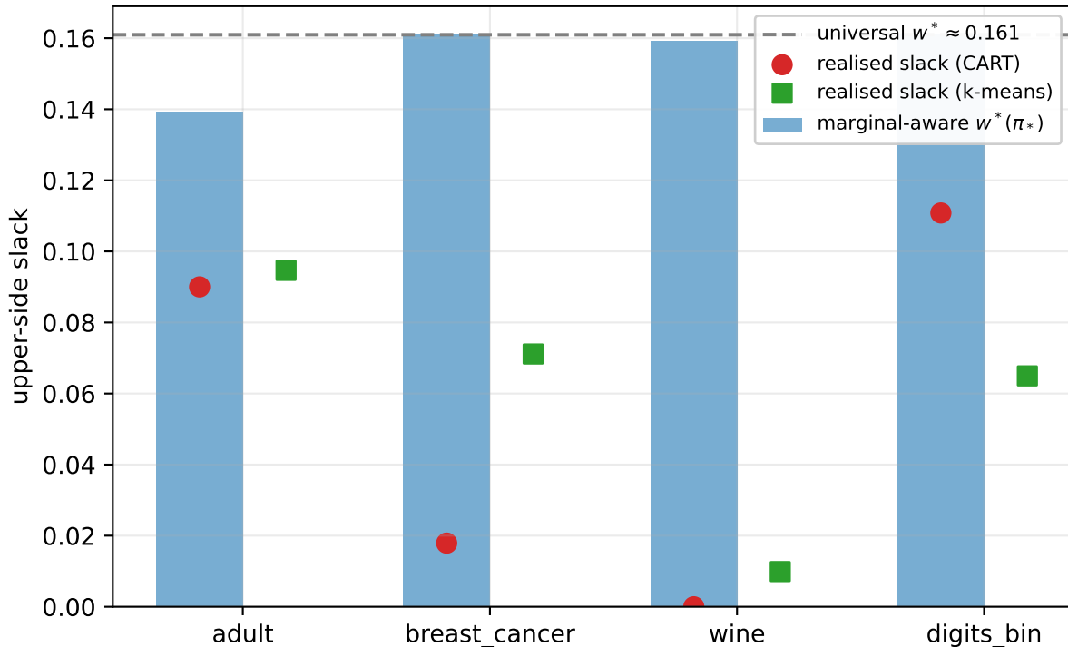
Marginal-aware slack shrinks the bracket on real binary labels
