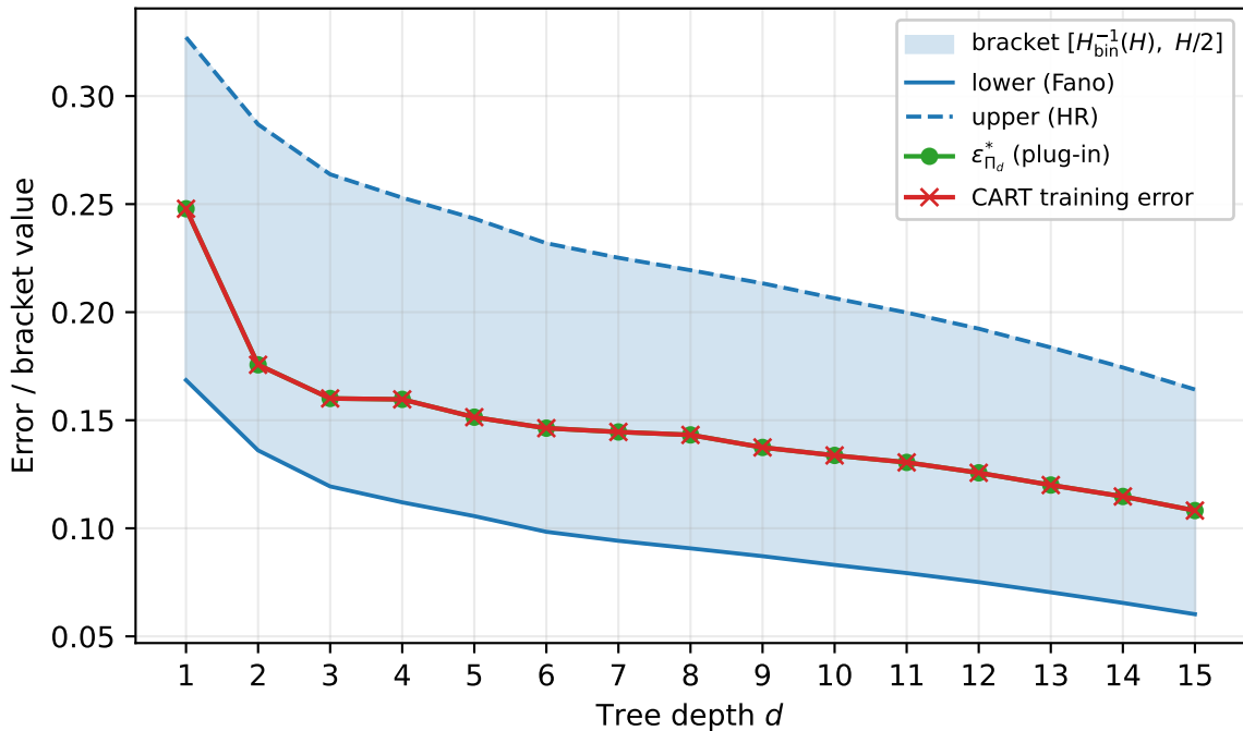
Refinement funnel on UCI Adult (depths 1..15)
