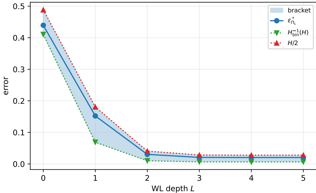
E3: WL bracket funnel — cora
