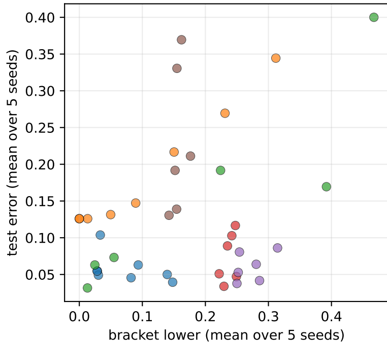
digits_bin \tau=+0.11 CI95=[-0.12,+0.31] speedup 1x
