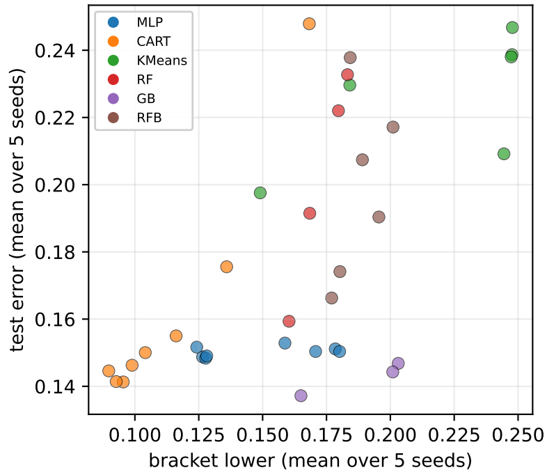
adult \tau=+0.48 CI95=[+0.25,+0.69] speedup 2x
