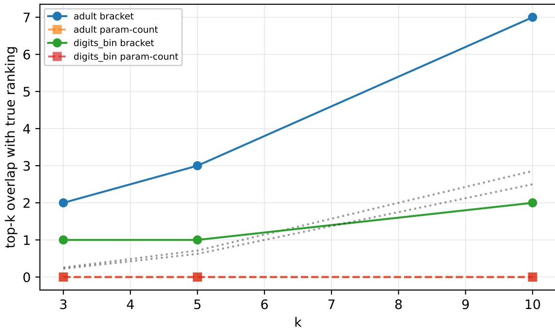
E6 NAS v2: top-k overlap (bracket vs param-count vs random)
