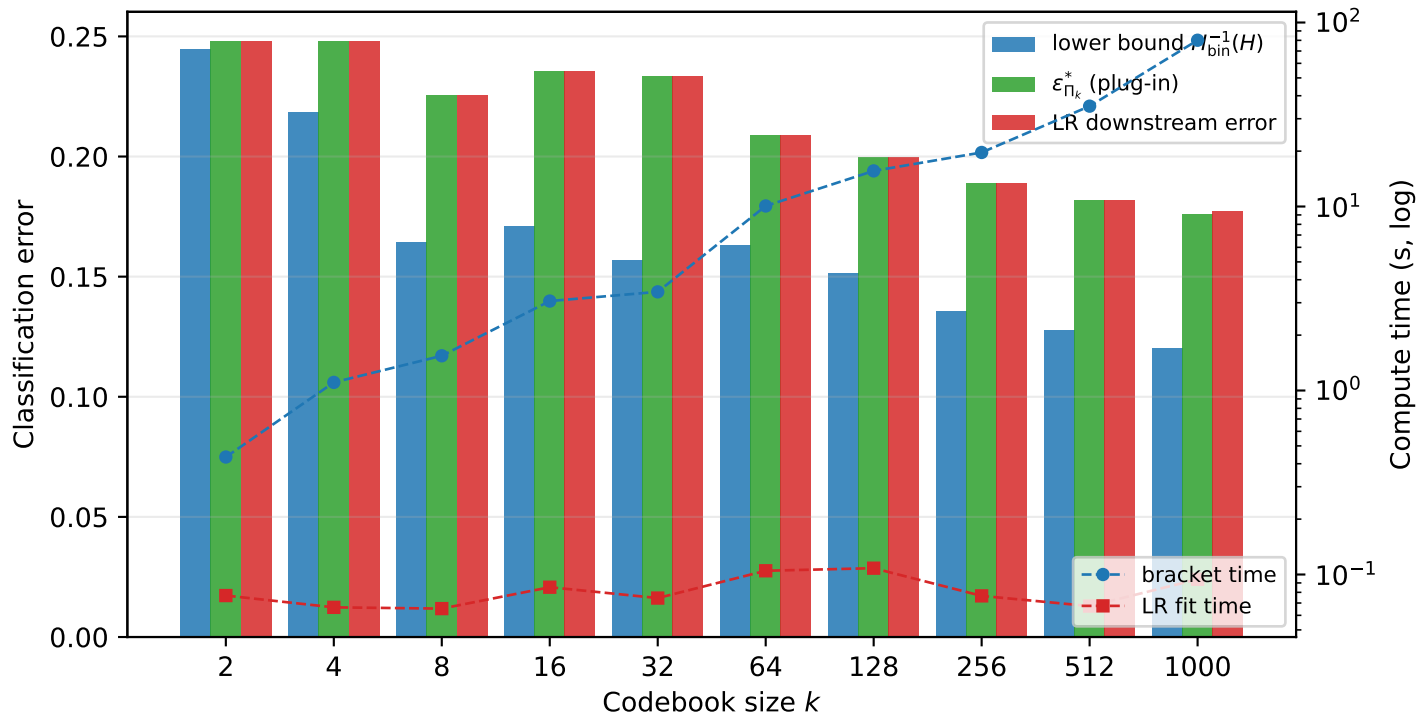
Zero-shot architecture selection on UCI Adult
