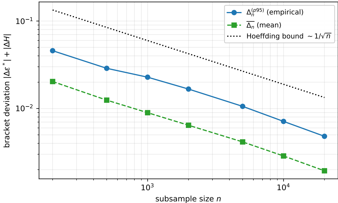
E7: empirical Proposition-7 concentration on UCI Adult
