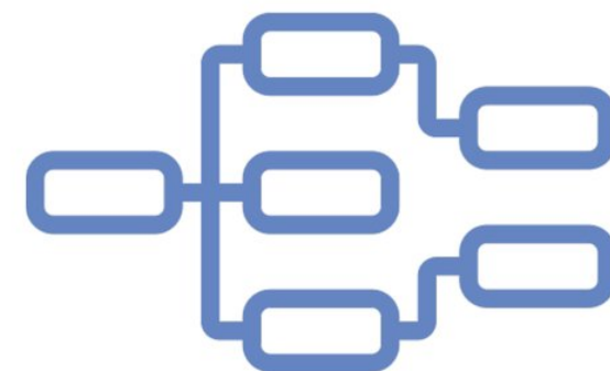
Event Loop
