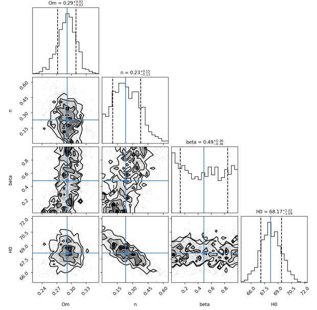
Figure 8. Corner plot showing posterior distributions and correlations between DVCH parameters from the full late-time MCMC analysis. Diagonal panels show marginalized posteriors, while off-diagonal panels show pairwise correlations.
