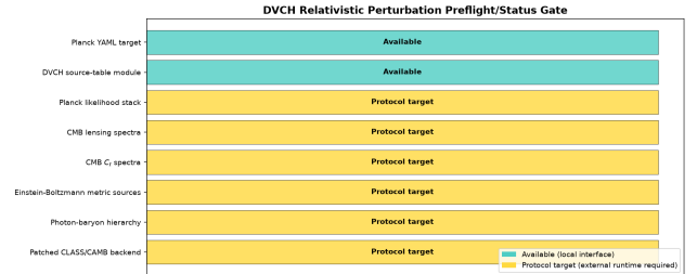
Figure 6. Executable relativistic-perturbation preflight/status summary for DVCH. Green entries denote local interface/configuration files that are present; yellow entries denote external CLASS/CAMB–Planck runtime inputs required before any CMB posterior can be quoted. The figure is a reproducibility/status diagnostic, not a new Planck posterior result.
