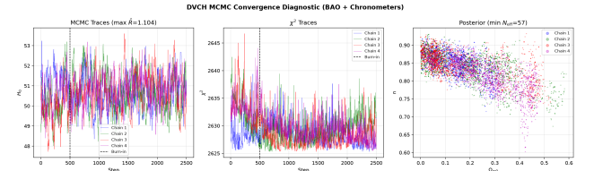
Figure 12. Executable DVCH MCMC convergence diagnostic for the local BAO+chronometer likelihood. The dashed line marks burn-in. The displayed chains are generated by dvch_mcmc_convergence.py and summarized by dvch_mcmc_convergence_summary.csv . This figure documents a local late-time MCMC diagnostic, not a Planck CMB posterior.
