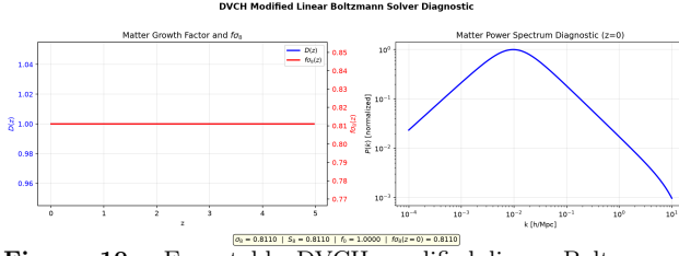
Figure 10. Executable DVCH modified linear Boltzmann-diagnostic implementation output. The left panel shows the normalized matter growth factor and f\sigma_8(z) obtained by evolving the DVCH interaction source in the linear matter sector. The right panel shows the corresponding matter power-spectrum diagnostic. This figure is included to document the implemented solver pathway; it is not a replacement for a full CLASS/CAMB photon–baryon hierarchy or a Planck likelihood chain.
