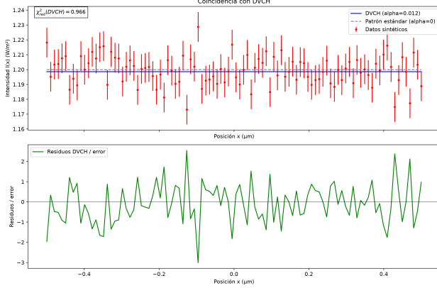
Figure 7. DVCH double-slit interference comparison. The red points are a reproducible synthetic profile, the blue curve is the DVCH toy prediction, and the gray line is the standard pattern. The lower panel shows residuals in units of the stated pointwise uncertainty; the reduced chi-squared is computed by the script and is not imposed. The axes are labeled "Posición x ( \mu\text{m} ), Intensidad I(x) ( \text{W}/\text{m}^2 )".
