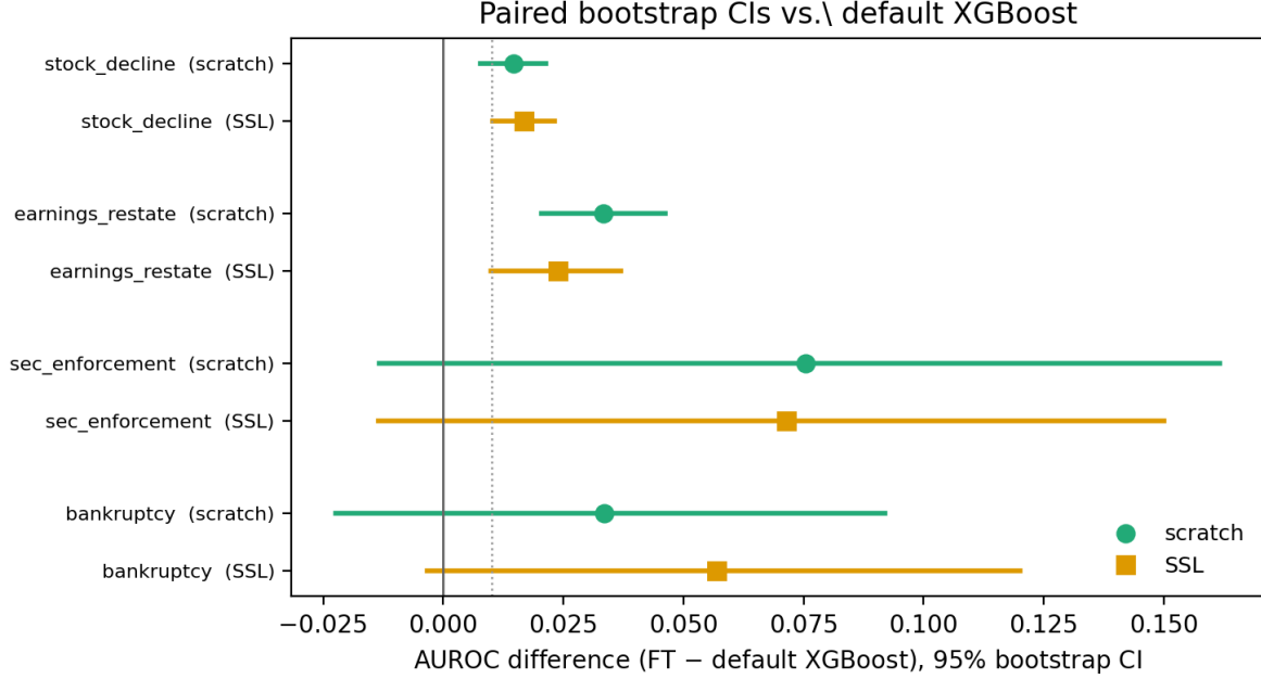
Figure 5: Paired bootstrap 95% CIs on AUROC difference (FT-Transformer minus default XGBoost, n = 1,000 resamples). The dashed line indicates the 0.01 gate margin. Green circles: FT tuned (scratch); yellow squares: FT tuned + SSL.
