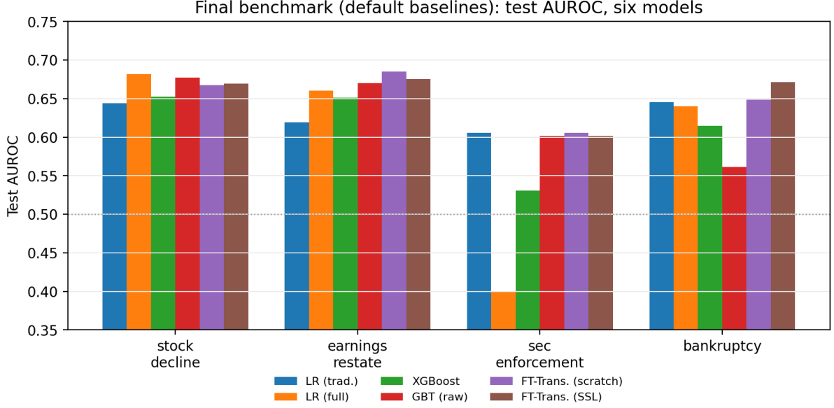
Figure 4: Final benchmark (default baselines): test AUROC for all six models across four distress outcomes.
