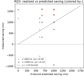
Figure 4: RQ3: per-question measured saving vs. the H bound for the same 60 questions, colored by tool latency L . Most points lie above y=x because the pipeline also hides query-generation latency, which H does not model. At L=600 ms (light) the bound saturates—59/60 points share H=600 ms; at L=1000 ms (dark) H spreads across \{0, 667, 1000\} ms, yet measured savings still do not track it (Spearman \rho = +0.12 ). The lone point below zero is a late-stabilizing query whose mis-fire the floored bound cannot express—and whose H is nonetheless maximal.
