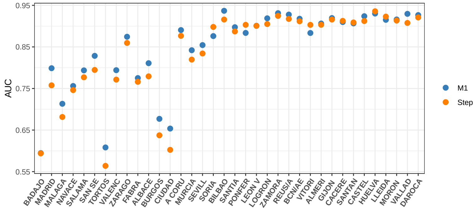
Comparison of AUCs of M1 versions
