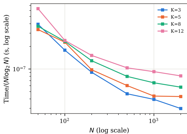
(b) Normalized running time ( \rho = 0 )
