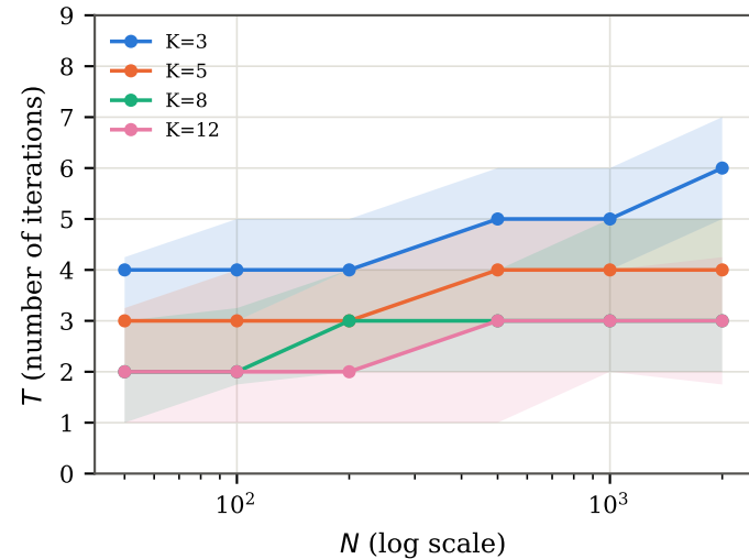
(a) Iterations T across 1,440 trials
