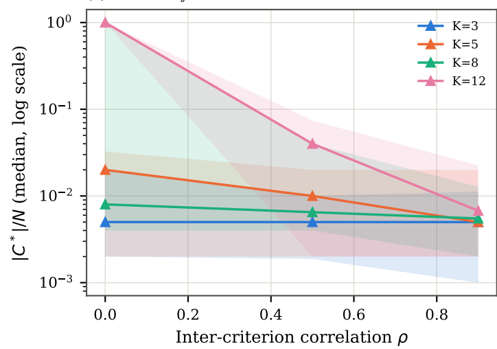
(c) Selectivity vs. criterion correlation
