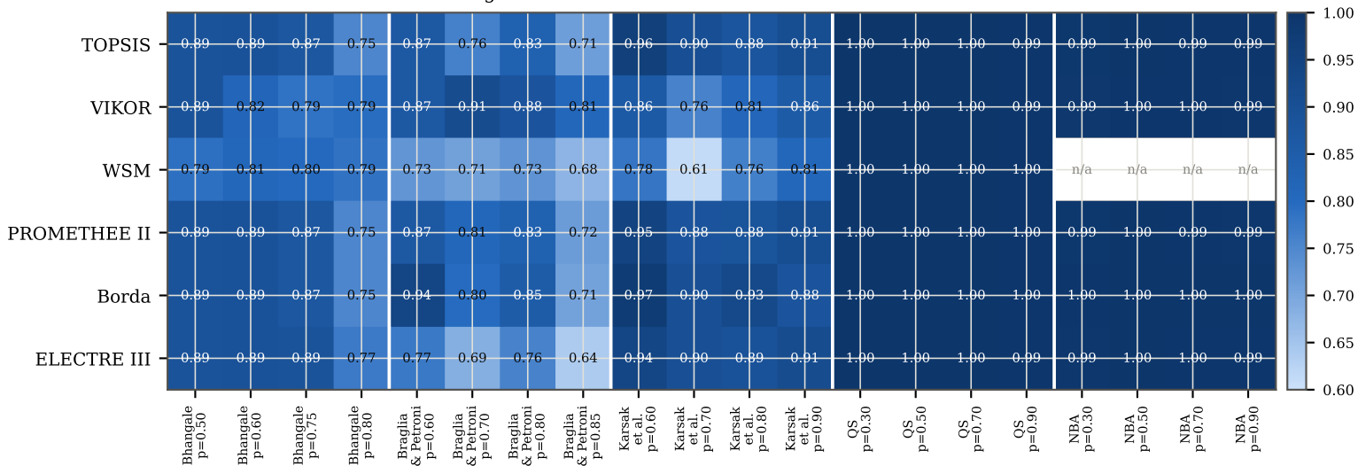
WS coefficient vs induced ranking
