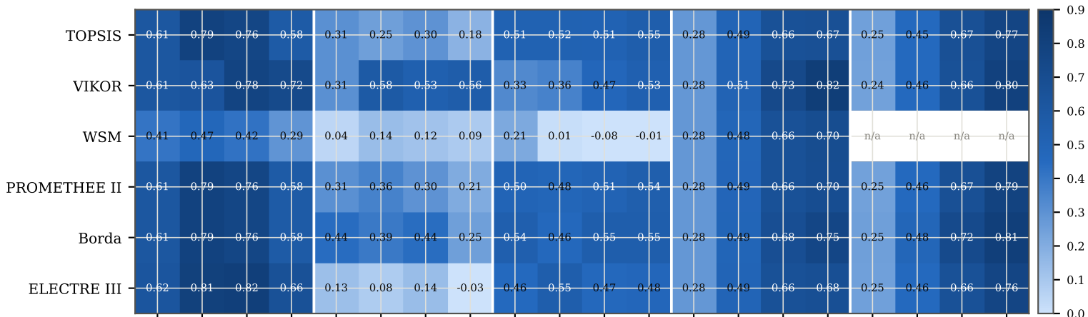
Spearman \rho vs induced ranking
