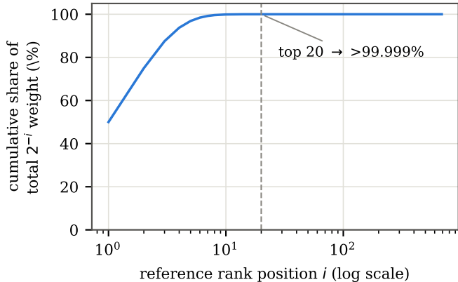
(a) WS weight concentration
