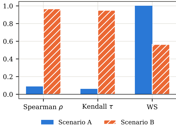
(b) Two disagreement patterns ( N = 690 )
