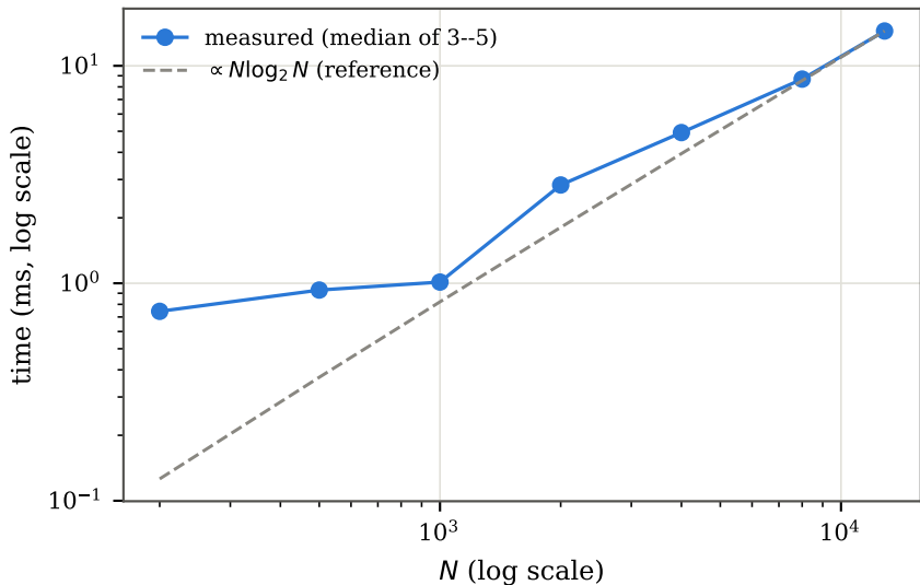
Empirical running time, full NBA panel (1996--2022, p = 0.7 , L = 1 )
