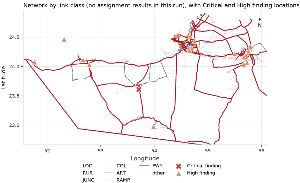
Network map: links by class (the run has no assignment results), Critical and High finding locations marked [src: links table (geometry_wkt, link_class); findings.json]
