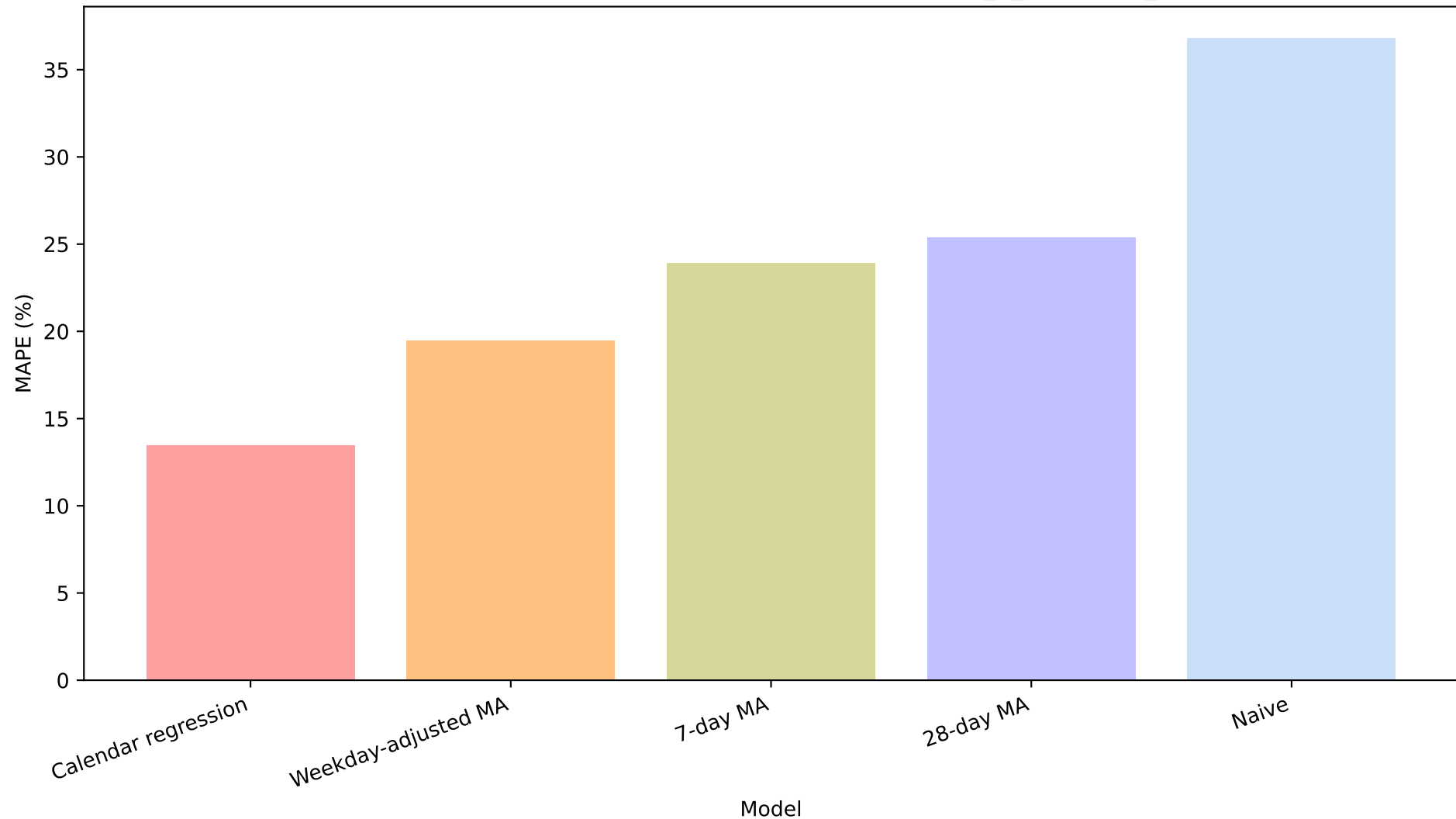
Forecast Model Comparison by MAPE (%): FOODS_3_586 at TX_2
