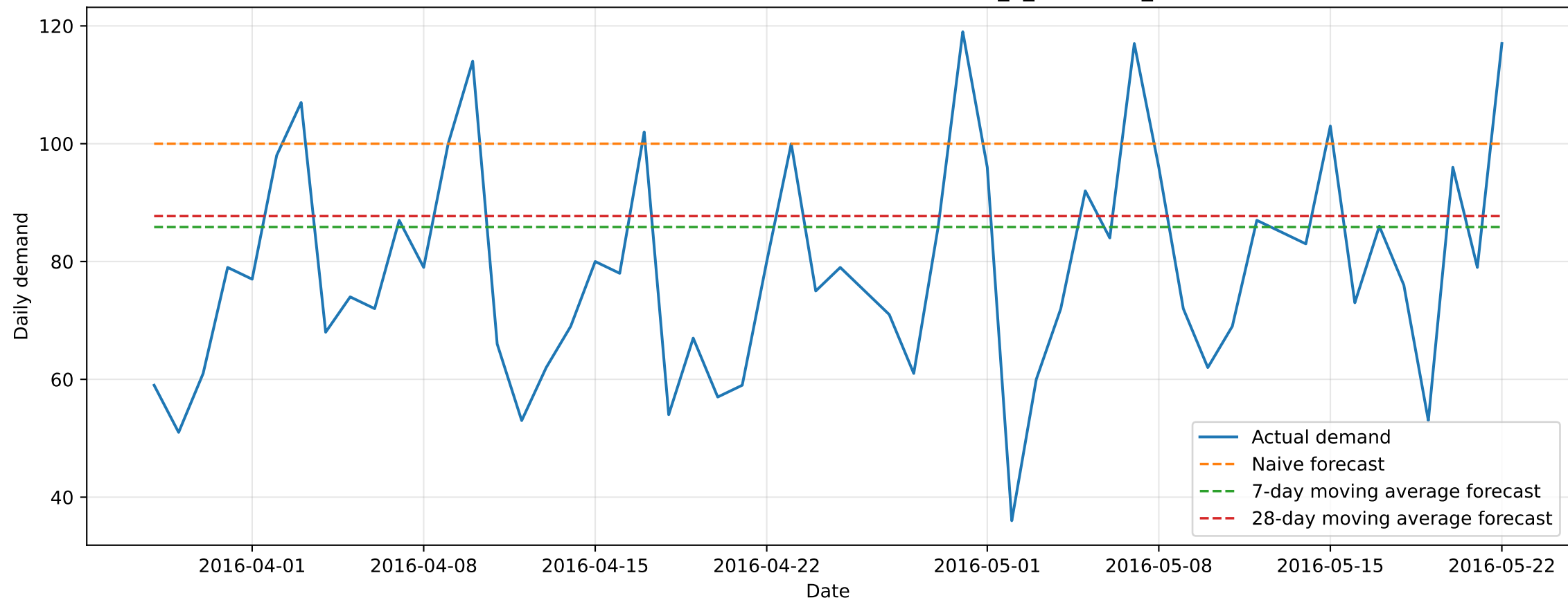
Baseline Forecasts vs Actual Demand: FOODS_3_586 at TX_2
