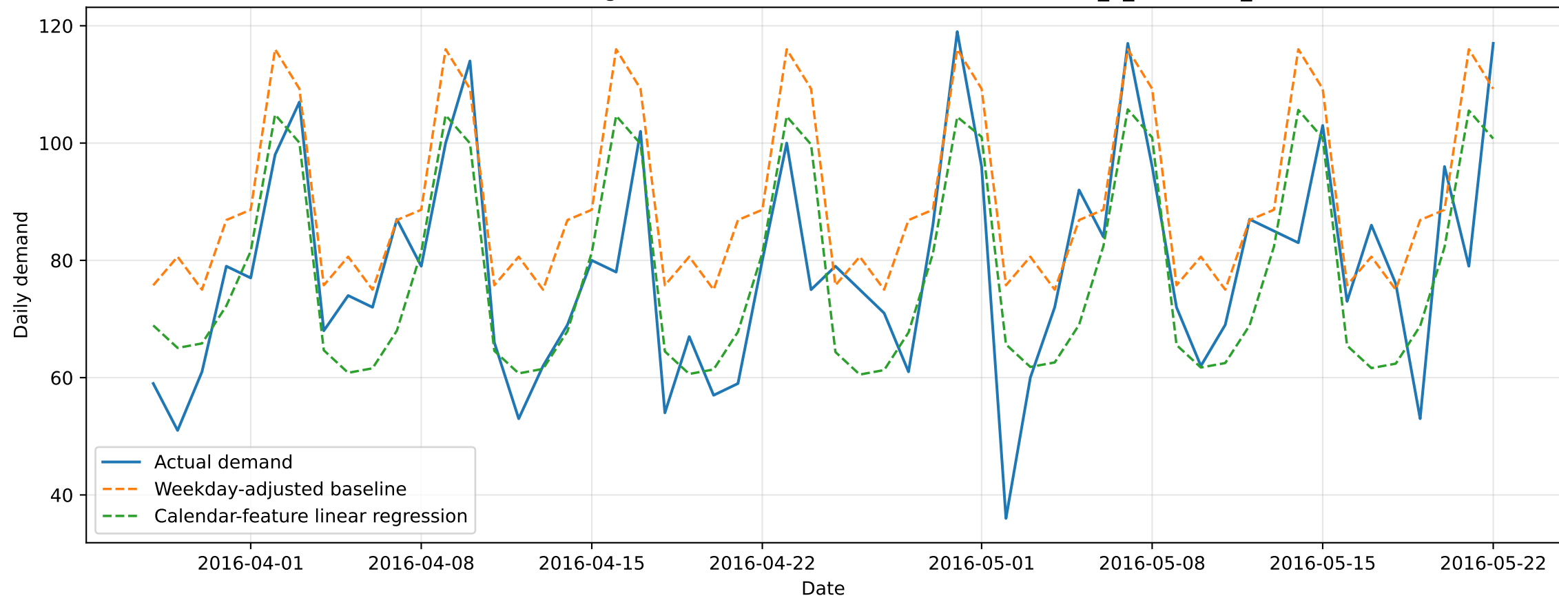
Calendar-Feature Regression Forecast vs Actual Demand: FOODS_3_586 at TX_2
