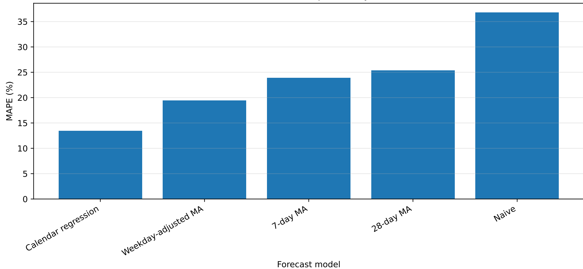
Forecast Model Comparison by MAPE
