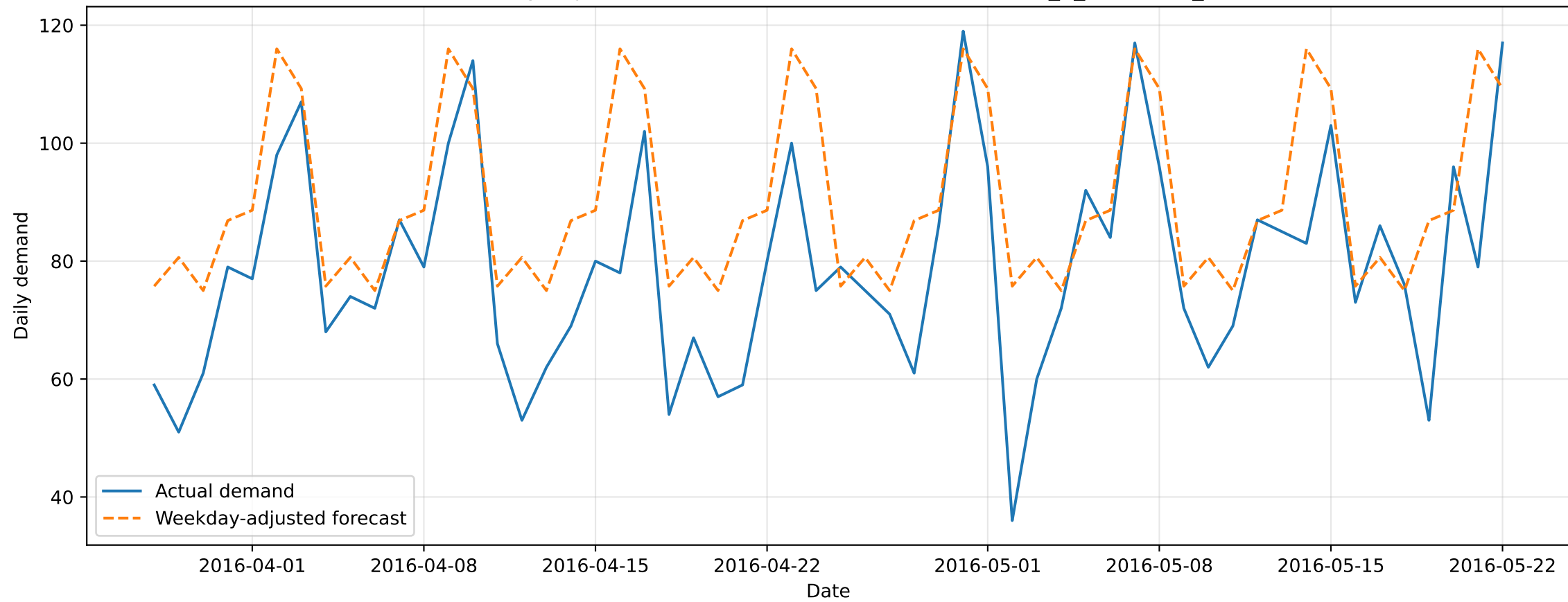
Weekday-Adjusted Forecast vs Actual Demand: FOODS_3_586 at TX_2
