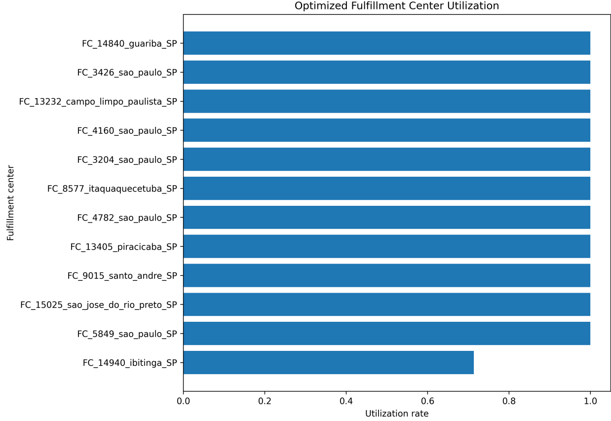
Figure 4: Optimized Fulfillment Center Utilization
