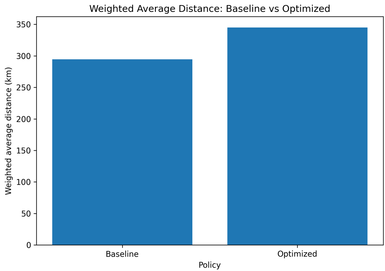
Figure 2: Weighted Average Distance
