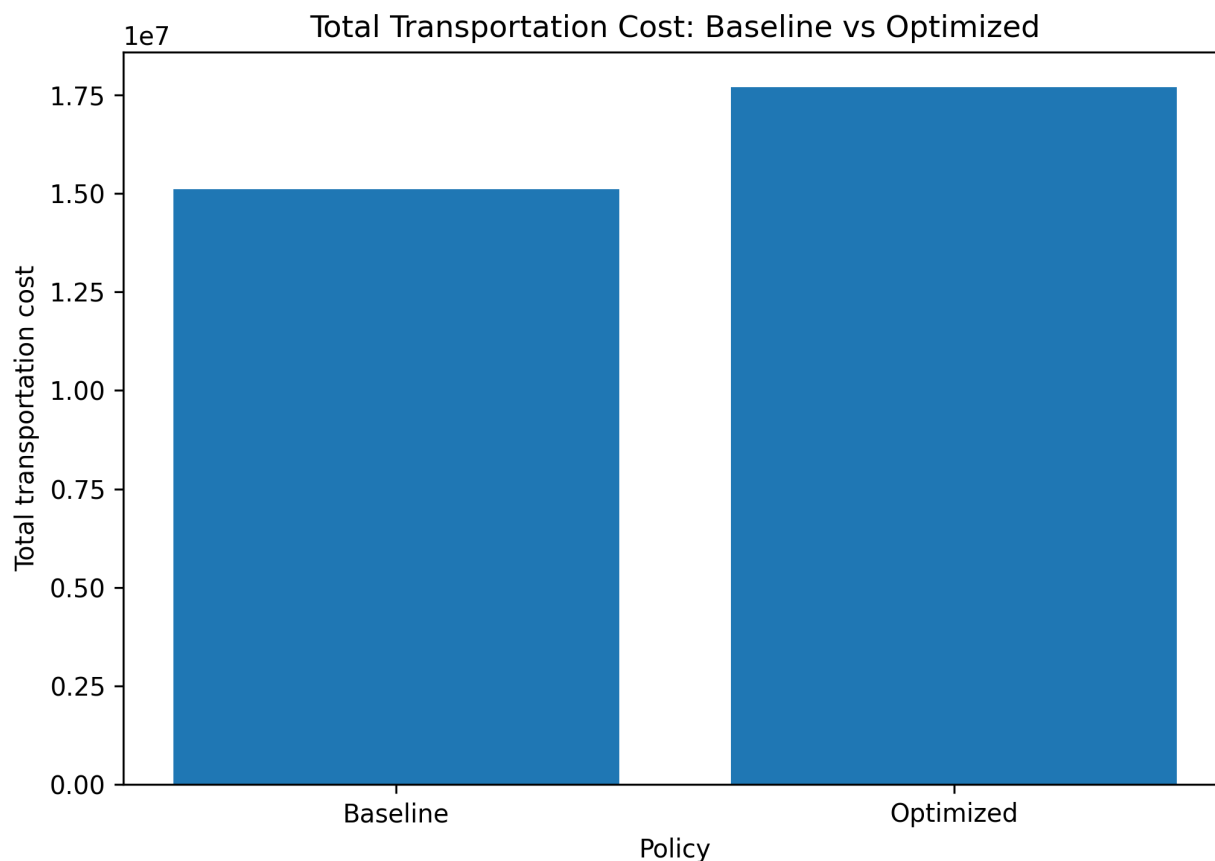
Figure 1: Total Transportation Cost
