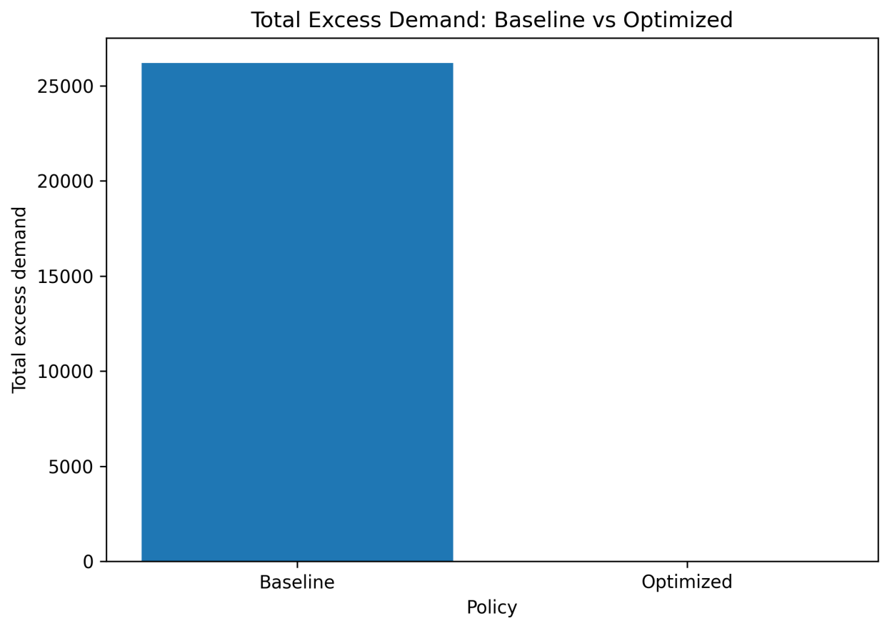
Figure 3: Total Excess Demand
