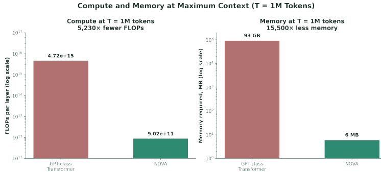
Figure 8: Compute and Memory at Maximum Context (T = 1M) — NOVA requires 5,230× fewer FLOPs and 15,500× less memory than a dense GPT-class Transformer.
