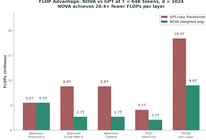
Figure 4: FLOP Comparison per Layer — NOVA achieves 20.4× fewer FLOPs than GPT at T = 64K.
