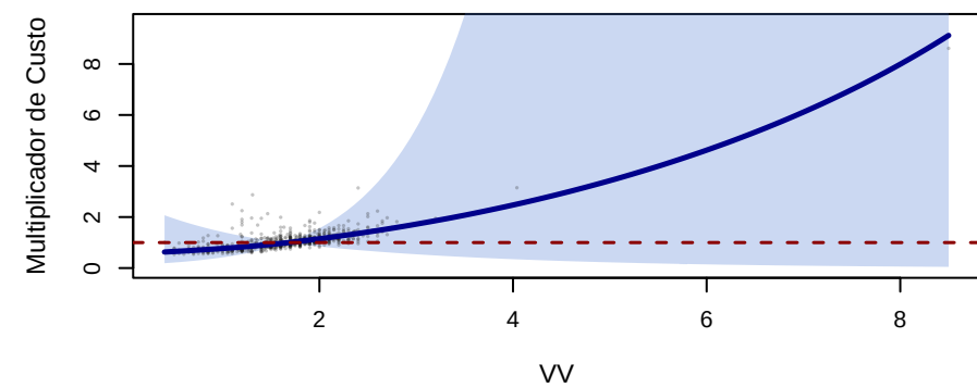
s(VV,2.79)
