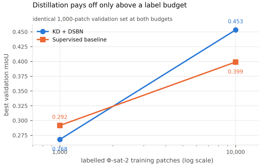
Figure 4.6: Best validation mIoU against labelled training budget. The two methods cross: distillation is worse at 1,000 labelled patches and better at 10,000. Both budgets share the same fixed validation split.
