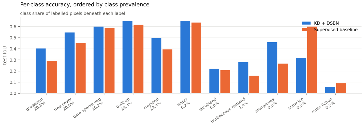
Figure 4.5: Per-class test IoU at 10,000 labelled patches, ordered by class prevalence. Distillation is ahead on nine of eleven classes. Neither model leaves any class unlearned, which unweighted cross-entropy did for four of them.
