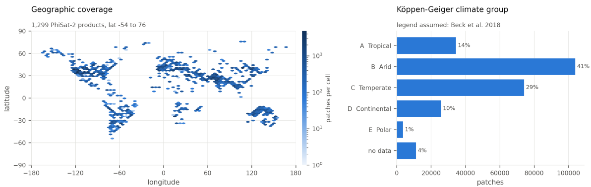
Figure 3.3: Left: spatial density of \Phi -sat-2 products (hexbin, log-scaled patch count per cell). Right: distribution of patches by Köppen–Geiger climate group[32].
