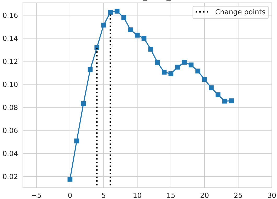
overall - drift_from_baseline
