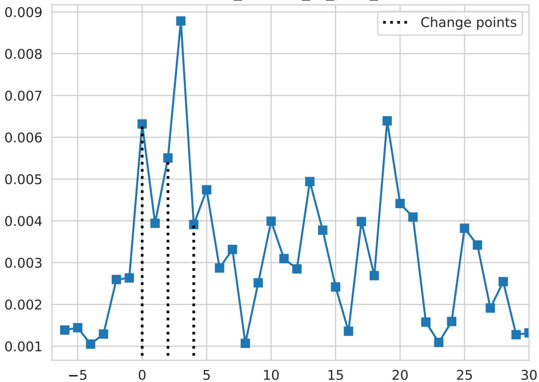
event - dist_smooth_to_prev_smooth
