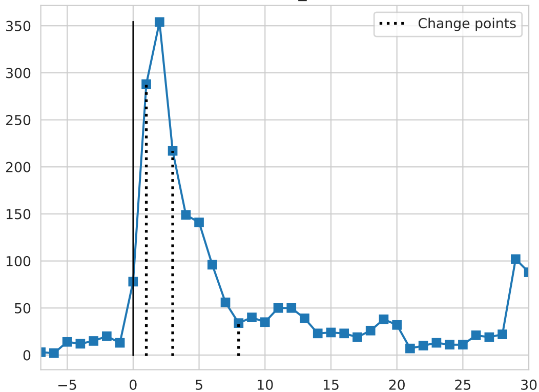
event - n_docs
