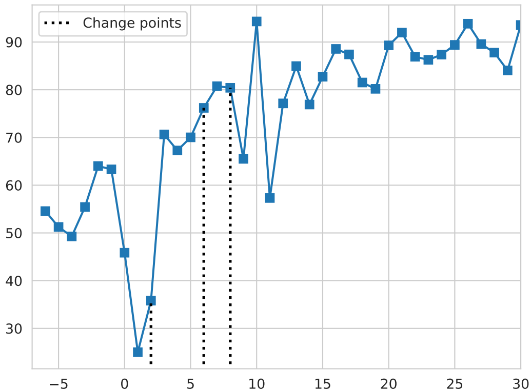
event - curvature
