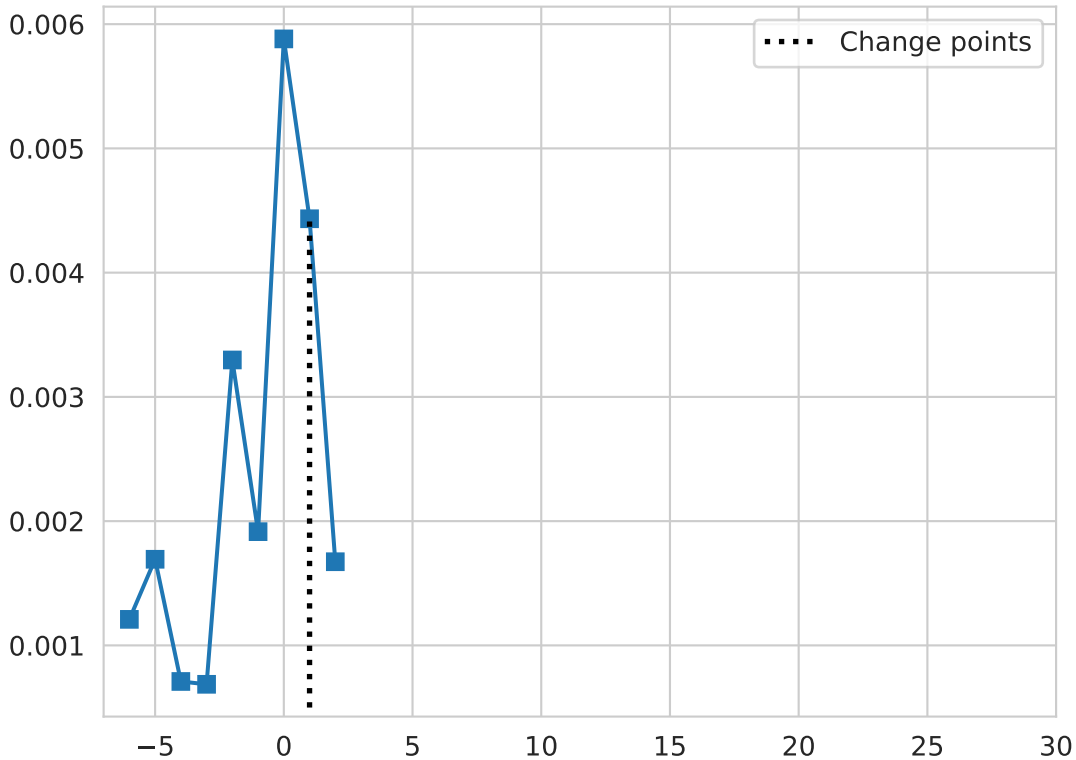
background - dist_smooth_to_prev_smooth
