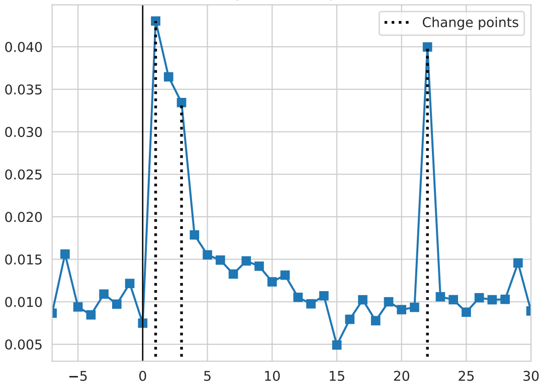
background - dispersion
