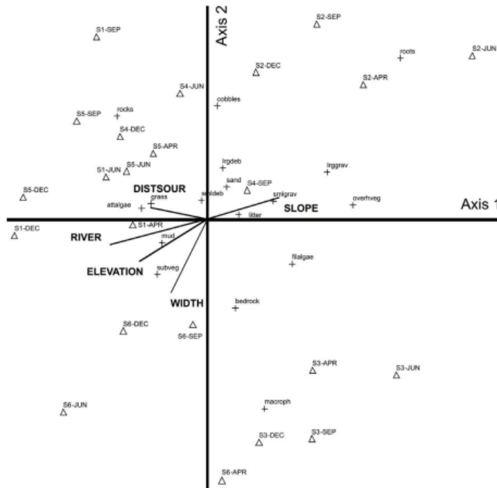
Figure 3. Biplot of ordination sites ( \Delta ) (based on CCA) in the catchment- and reach-scale variables space, as defined by CCA. Vectors represent river length (RIVER), distance of site from source (DISTSOUR), elevation, margin slope (SLOPE) and site width (WIDTH). (+) indicates position of habitat elements in the ordination space.
