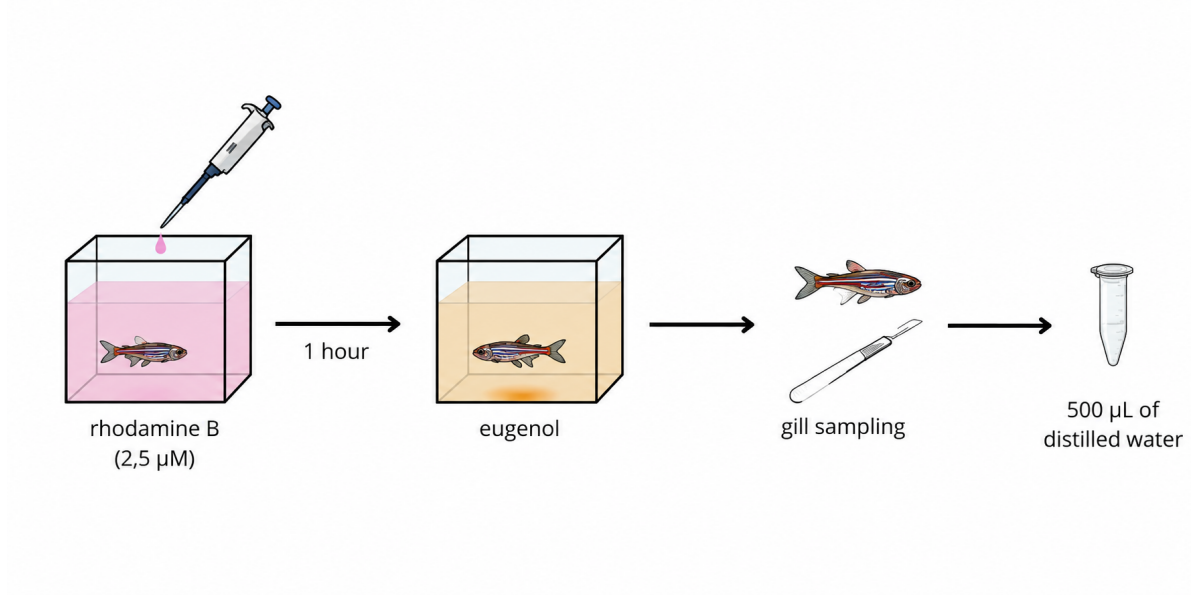
Figure 3: Experimental design of the procedure used to evaluate rhodamine B uptake in fish. The individuals were exposed to a rhodamine B solution (2.5 \mu\text{M} ) for 1 hour in an aquarium containing pink-colored water. Subsequently, the fish were anesthetized with eugenol for gill sampling. The collected material was placed in microtubes containing 500 \mu\text{L} of distilled water for later analysis.
