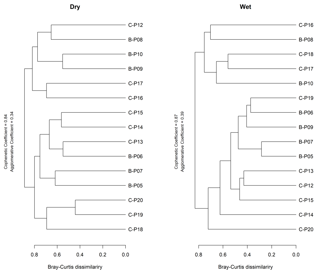
Figure 5: UPGMA Classification
