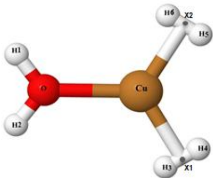
Figure 6. Optimized geometry of \text{Cu}^+(\text{H}_2\text{O})(\text{H}_2)_2 at the CCSD(T)/aug-cc-pVTZ(-PP) level and definition of geometry parameters. X1 and X2 represent the centers of mass of \text{H}_2 ligands.
