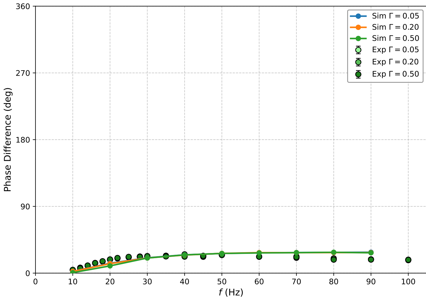
Phase Validation Overlay (sweep_original)
